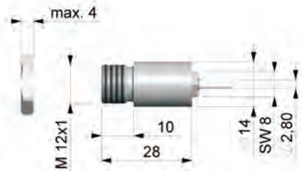
Dimensions CSmicro
