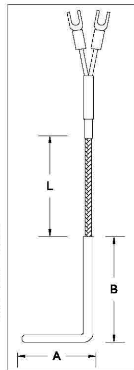
BASIC WIRE THERMOCOUPLE WITH 90 DEG BEND
