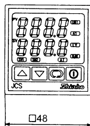
8.2 External dimension drawing One-touch type mounting bracket
