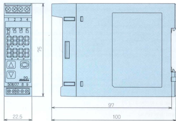
External dimension
