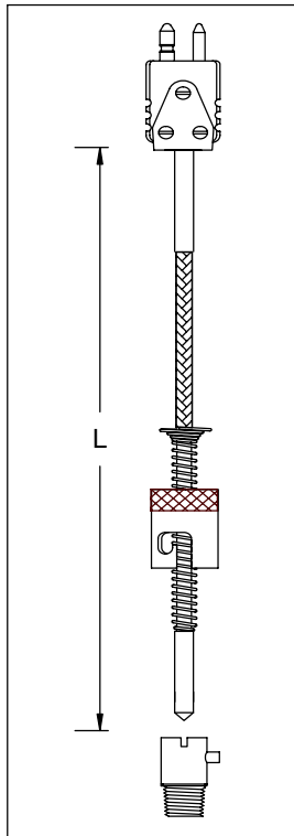
LARGE PLUG FITTED TO BAYONET CAP THERMOCOUPLE
