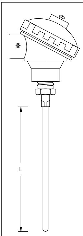
MODEL TC06 BASIC ASSEMBLY LARGE ALUMINIUM TERMINAL HEAD
