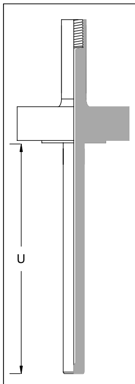
PARALLEL STEM RAISED FACE FLANGED THERMOWELL
