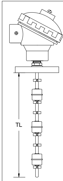
FLANGED LEVEL SWITCH THREE SMALL FLOATS
