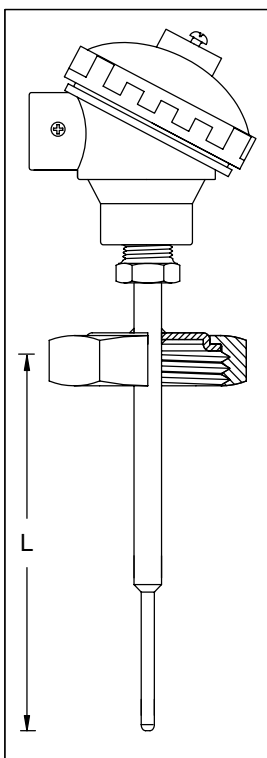
BSM PROCESS CONNECTION HYGIENIC WELDS REDUCED TIP
