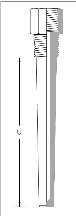
TAPERED STEM BAR STOCK THERMOWELL
