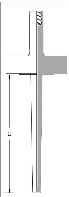
TAPERED STEM RAISED FACE FLANGED THERMOWELL
