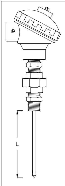
SPRING LOADED NIPPLE/UNION/NIPPLE CONNECTION FOR EASY REMOVAL
