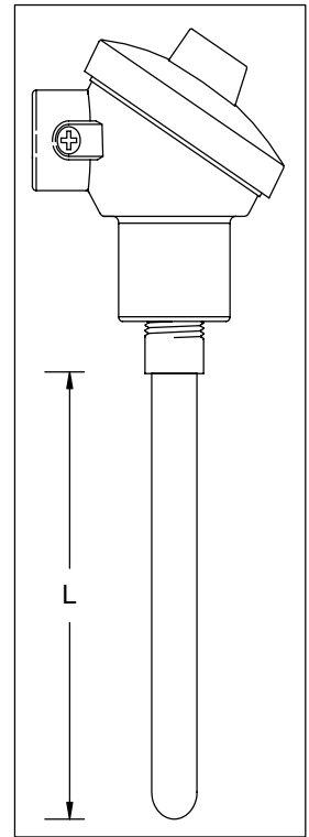
CERAMIC SHEATH PROBE WITH SMALL ALUMINIUM TERMINAL HEAD
