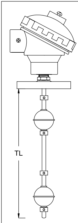
FLANGED LEVEL SWITCH DUAL LARGE FLOATS
