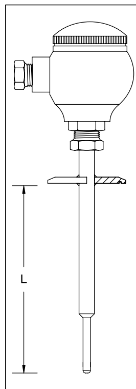
STAINLESS STEEL BAKELITE OR POLYPROPYLENE HEAD
