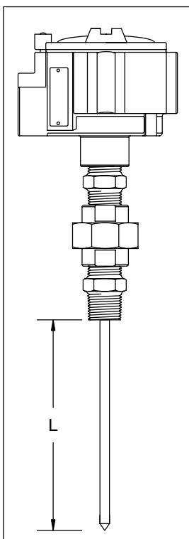
SAA Ex d CLASS 1 ZONE 1 FLAME PROOF ASSEMBLY
