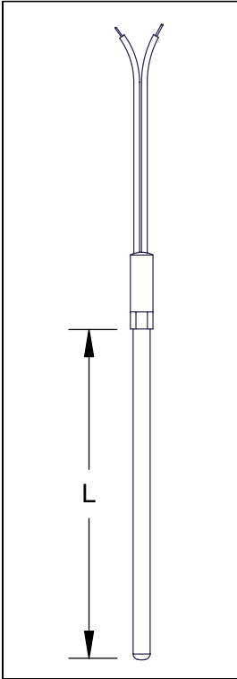
BASIC MIMS THERMOCOUPLE C/W POT SEAL
