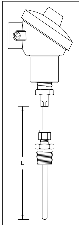
MODEL TC01 C/W MALE CONNECTOR BRASS/ STAINLESS STEEL NPT/BSP THREAD
