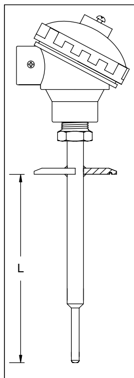
TRICLOVER PROCESS CONNECTION HYGIENIC WELDS REDUCED TIP
