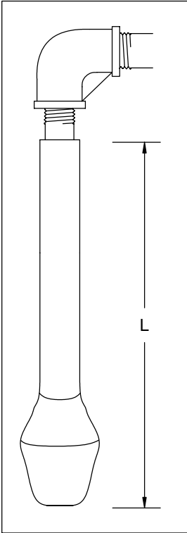
LAMINATED AND REFRACTORY SHEATH SUITABLE FOR DIECASTING
