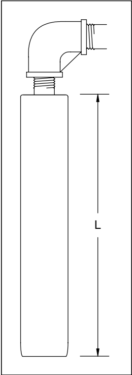
VESUVIUS SHEATH SUITABLE FOR DIECASTING
