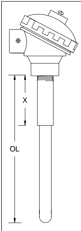
HIGH TEMPERATURE THERMOCOUPLE CERAMIC SHEATH AND HOLDING TUBE
