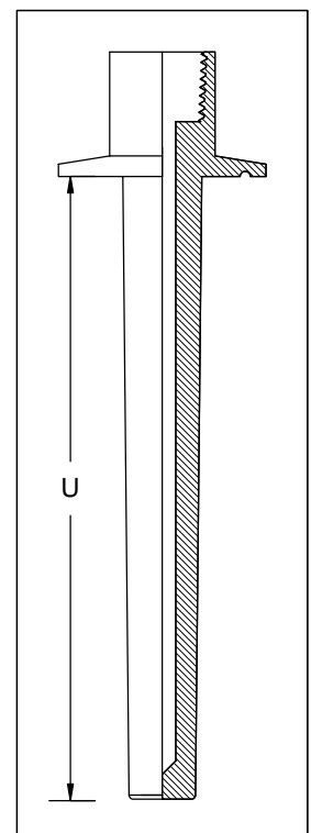
316SS THERMOWELL WITH TRICLOVER FLANGE
