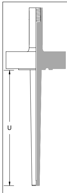
TAPERED STEM RJT RING JOINT TYPE FLANGED THERMOWELL
