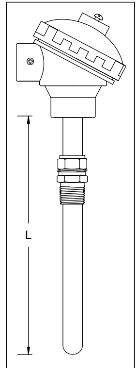
NOMINAL BORE HEAVY WALL PIPE PROTECTION SHEATH INCONEL / 253MA
