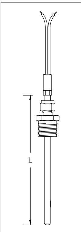
BASIC MIMS THERMOCOUPLE C/W CONNECTING TAILS
