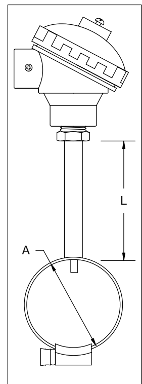
Ex ia SENSOR FOR PIPE SURFACE MEASUREMENT
