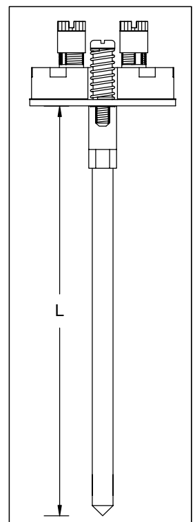
SPRING LOADED TERMINAL BLOCK SUITS 33mm CENTRES
