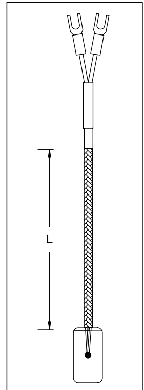
LEAF STYLE SENSOR TO FIT UNDER HEATING ELEMENT
