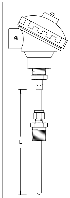
MODEL TC06 C/W MALE CONNECTOR BRASS/STAINLESS STEEL NPT/BSP THREAD
