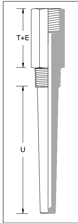
TAPERED STEM BAR STOCK THERMOWELL C/W LAGGING EXTENSION
