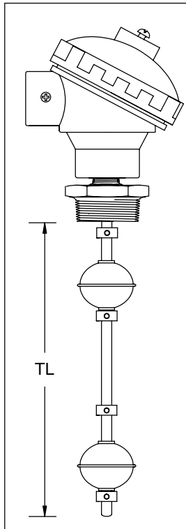
SCREWED CONNECTION LEVEL SWITCH DUAL LARGE FLOATS
