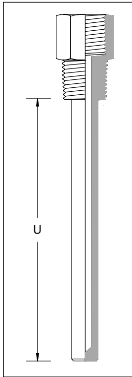
PARALLEL STEM BAR STOCK THERMOWELL
