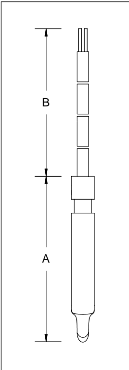
MARSHALL 446 LANCE PROBES NON FERROUS CASTING
