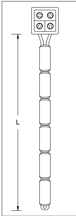
8 AWG OR 14 AWG BEADED THERMOCOUPLE WITH TERMINAL BLOCK
