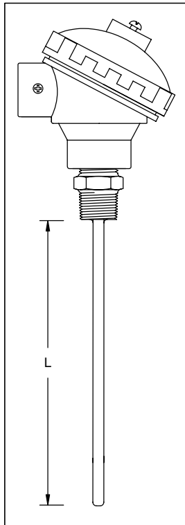
SPRING LOADED OR WELDED HEX NIPPLE CONNECTION
