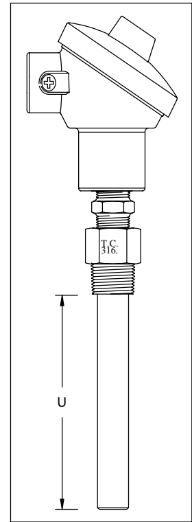
HEX NIPPLE CONNECTION WITH BARSTOCK THERMOWELL
