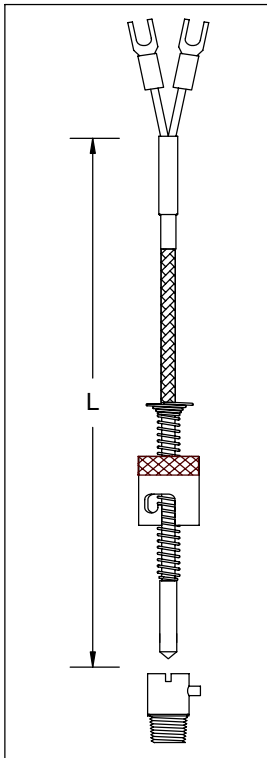
ADJUSTABLE YM3 BAYONET CAP THERMOCOUPLE C/W ADAPTOR
