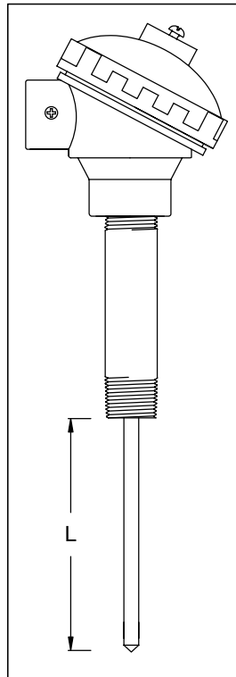
SPRING LOADED OR WELDED PIPE NIPPLE CONNECTION
