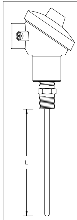
HEX NIPPLE CONNECTION FIXED / WELDED SPRING LOADED
