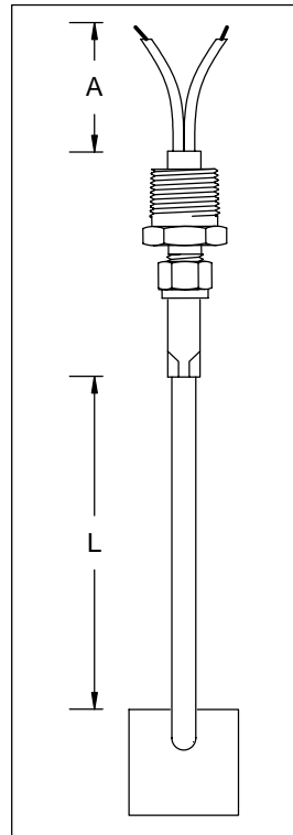
PAD STYLE MALE CONNECTOR FOR BULKHEAD CONNECTION
