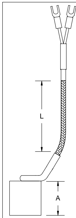
NOZZLE THERMOCOUPLE 1mm SHIM
